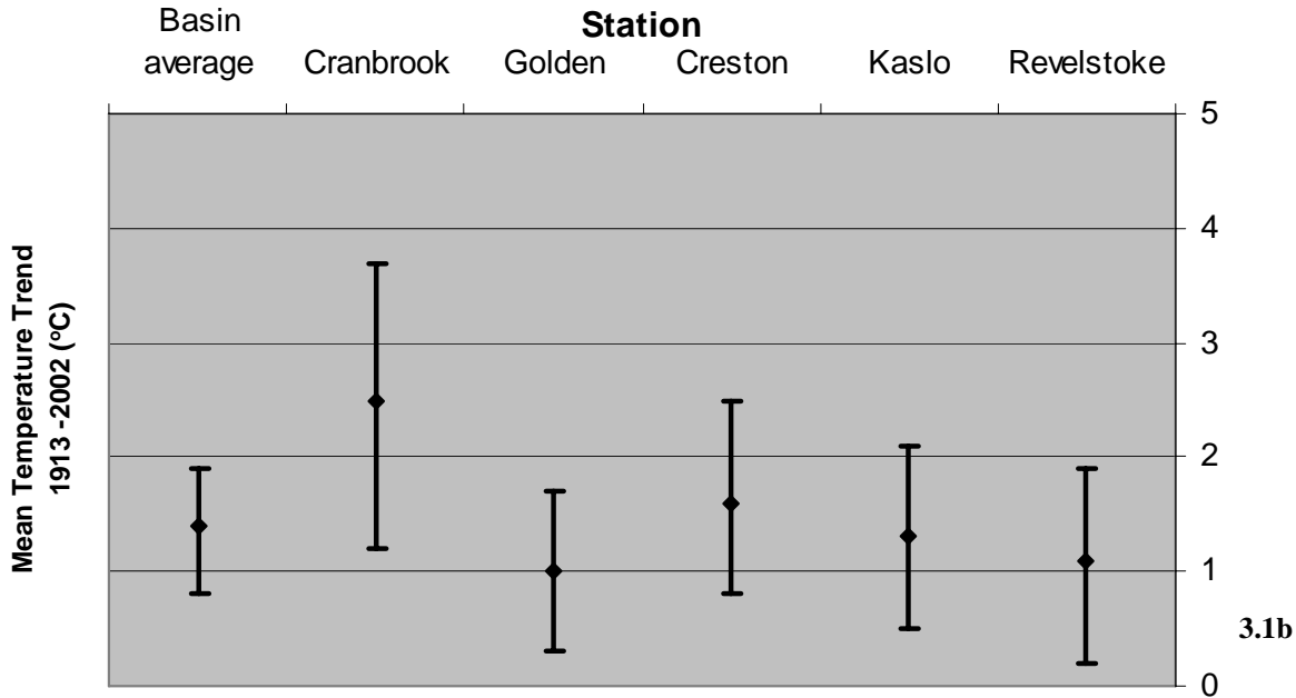
Figure 3.1: (b) Annual mean temperature trends and confidence intervals for each station and Basin average 1913-2002.
