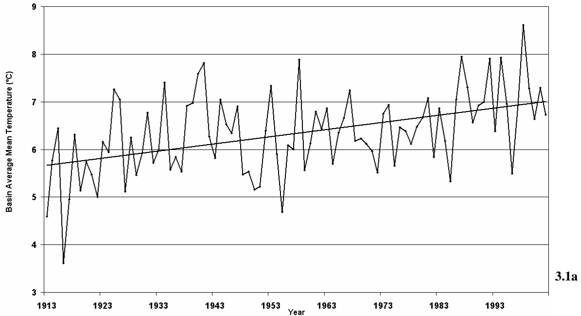
Figure 3.1: (a) Annual mean temperature record and trend for the Basin 1913-2002
