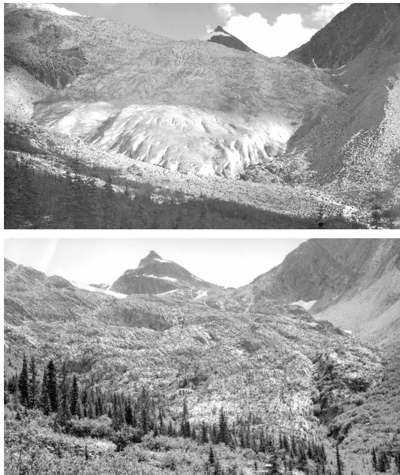
Figure 4.1 Retreat of the Illecillewaet Glacier between 1902 – 2002. Source: Dr. Henry Vaux.
