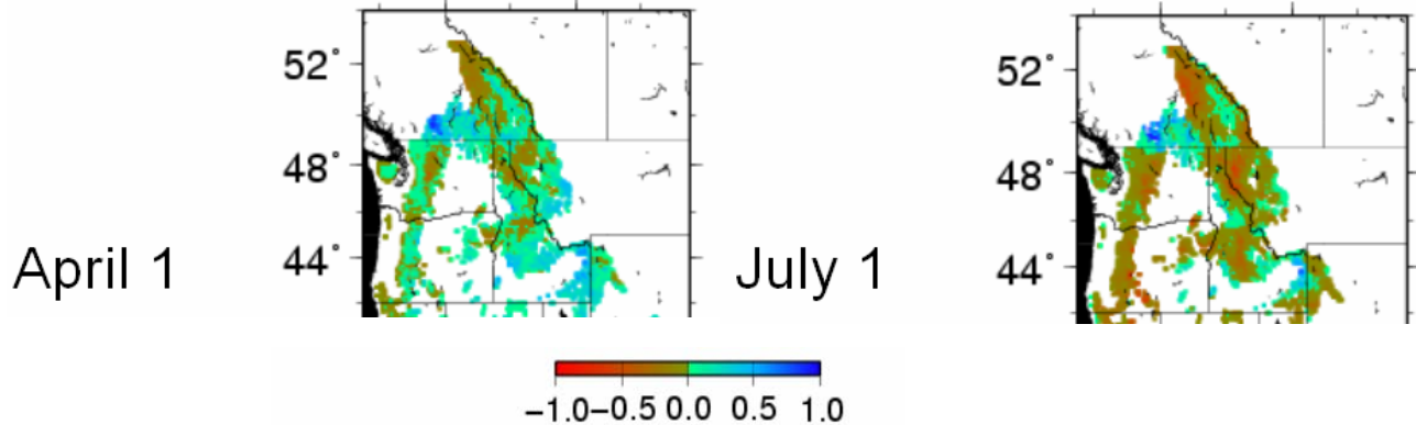
Figure 4.4: Soil Moisture Content trends from VIC 1947-2003 (% per year). Source: Climate Impacts Group, University of Washington.
