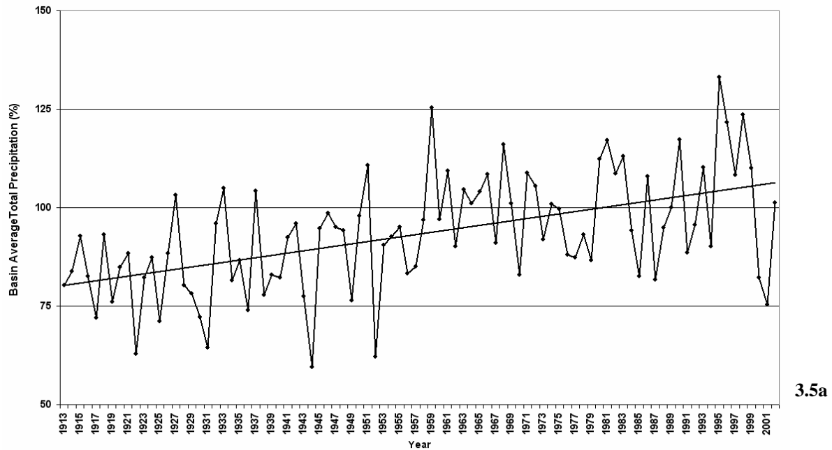
Figure 3.5: (a) Annual precipitation record and trend for the Basin 1913-2002 (b) Annual precipitation trends and confidence intervals for each station and the Basin average 1913-2002.
