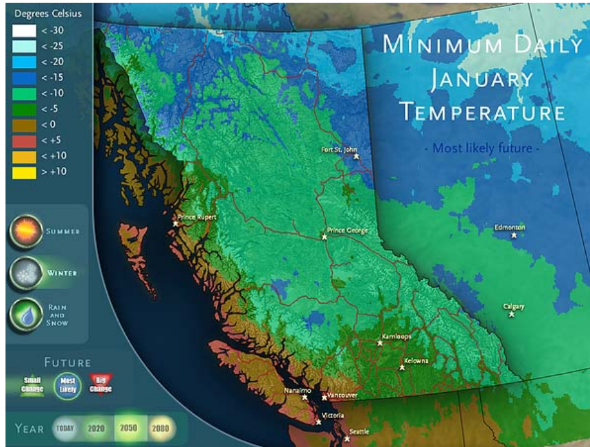
Figure 3.4: (f) High Resolution Temperature 2050s median Projection: January Mean Monthly Nighttime Low
