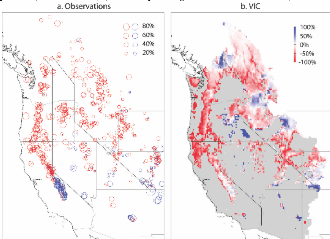
Figure 3.10: Observed snowfall trends and VIC model trends for April 1 Snow Water Equivalent (Mote et al. , 2005). (Values are percentages relative to current climate).
