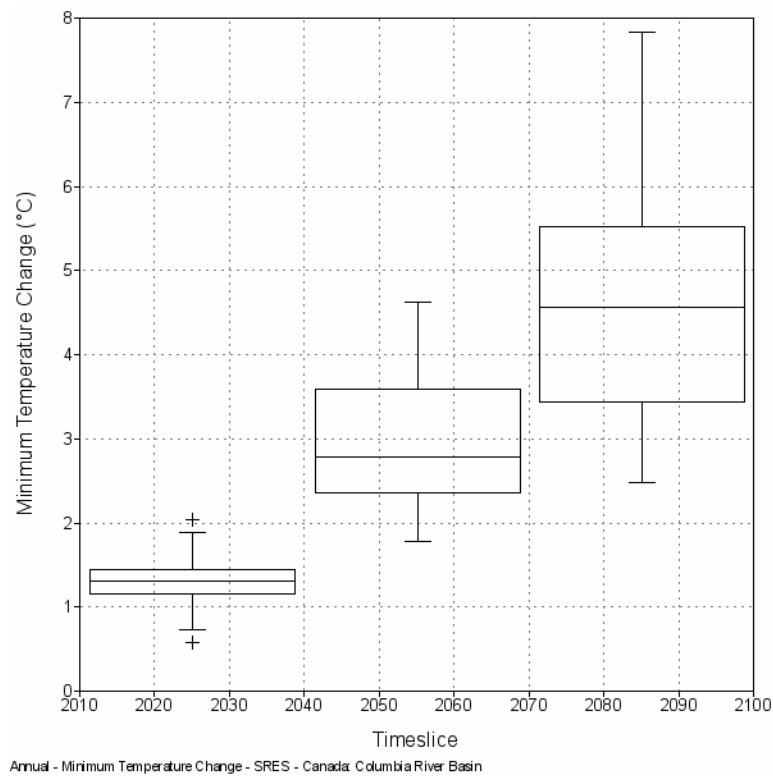
Figure 3.4: (b) Annual minimum temperature projections for the Basin 2020s, 2050s, and 2080s (c) High Resolution Temperature Baseline: July Mean Monthly Daytime High
