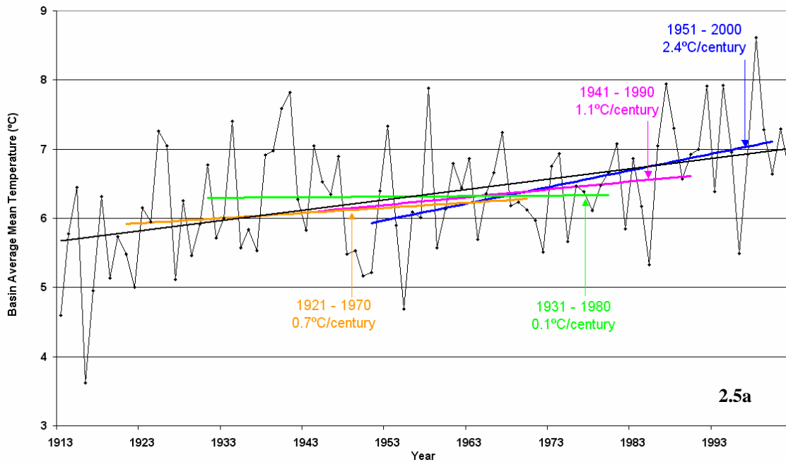
Figure 2.5: (a) Basin average annual mean temperature record and 50-year trends (b) Basin average annual mean temperature record and 30-year trends.
