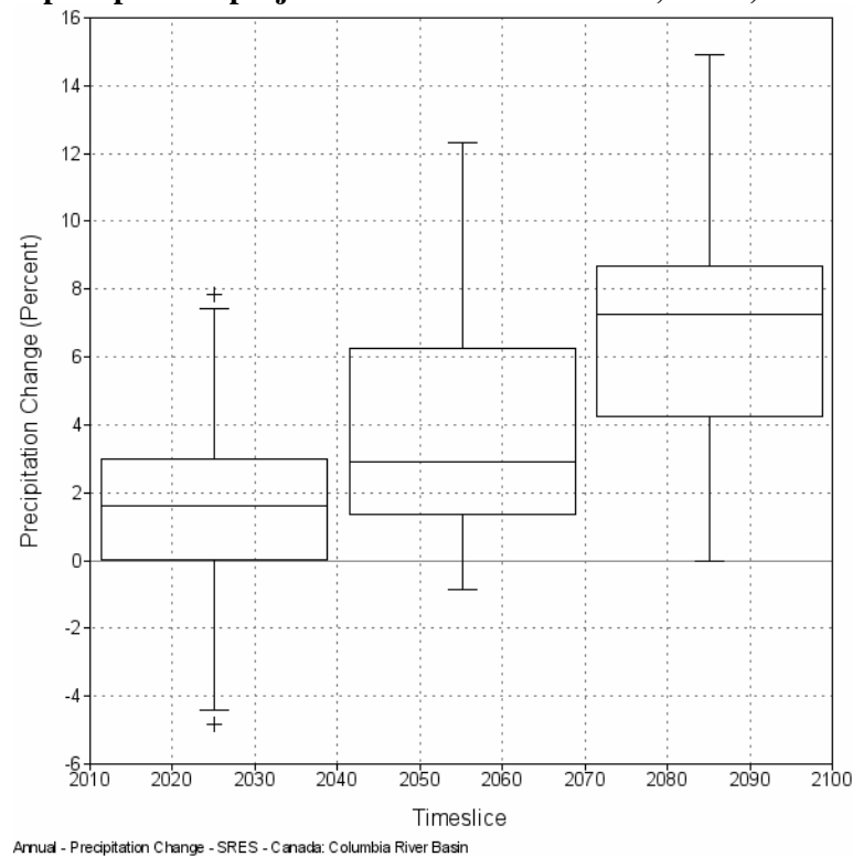
Figure 3.6: Annual precipitation projections for the Basin 2020s, 2050s, and 2080s
