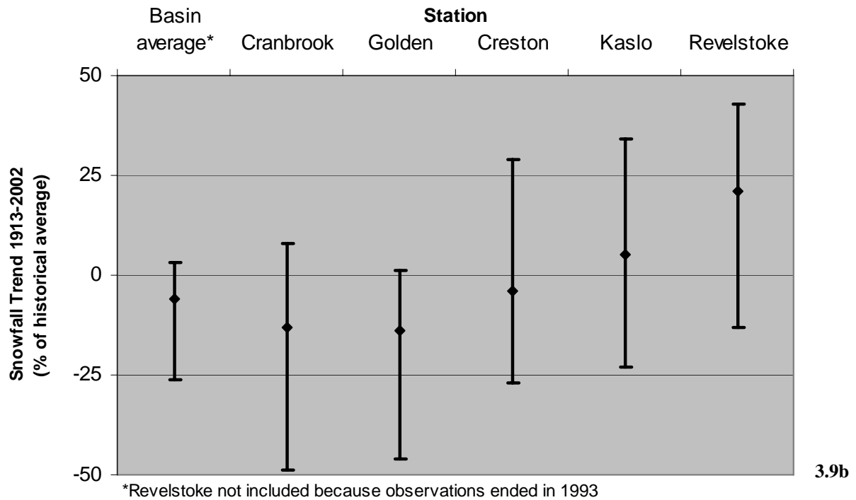
Figure 3.9: (b) Annual snowfall trends and confidence intervals for each station and Basin average 1913-2002
