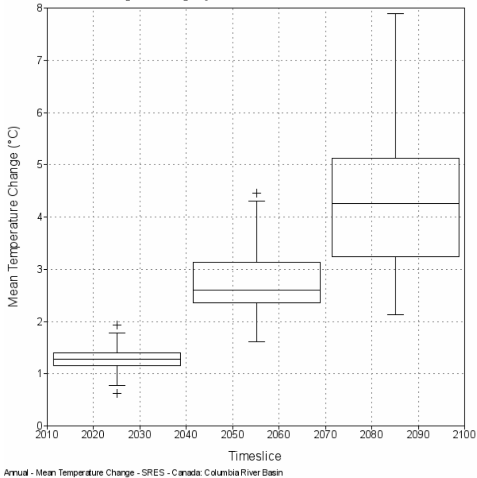
Figure 3.2: Annual mean temperature projections for the Basin 2020s, 2050s, and 2080s
