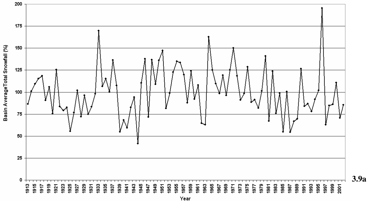
Figure 3.9: (a) Annual snowfall record and trend for the Basin 1913-2002
