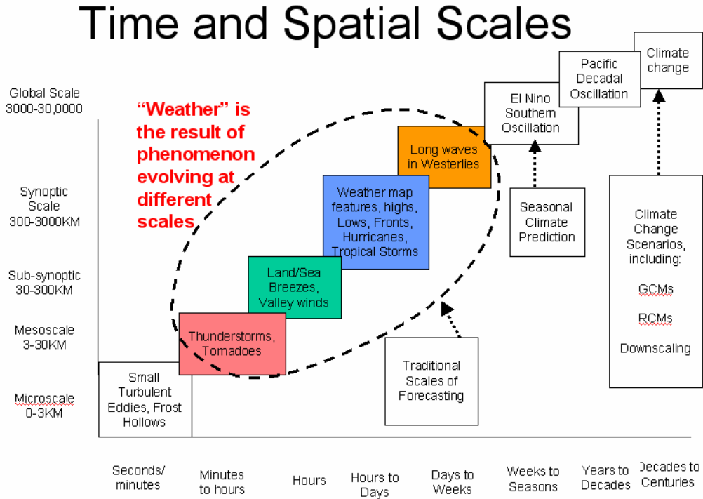
Figure 2.1: Time scales of weather and climate
