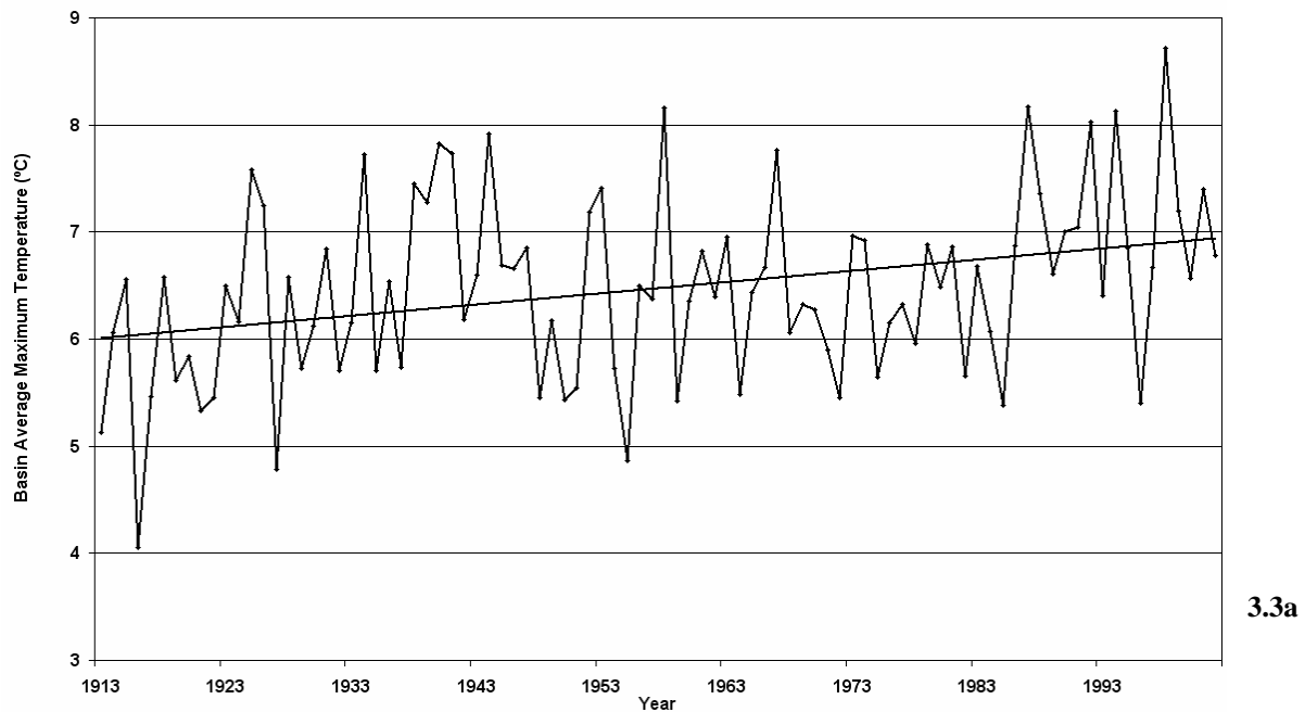
Figure 3.3: (a) Annual maximum temperature record and trend for the Basin 1913-2002 (b) Annual maximum temperature trends and confidence intervals for each station and Basin average 1913 – 2002.
