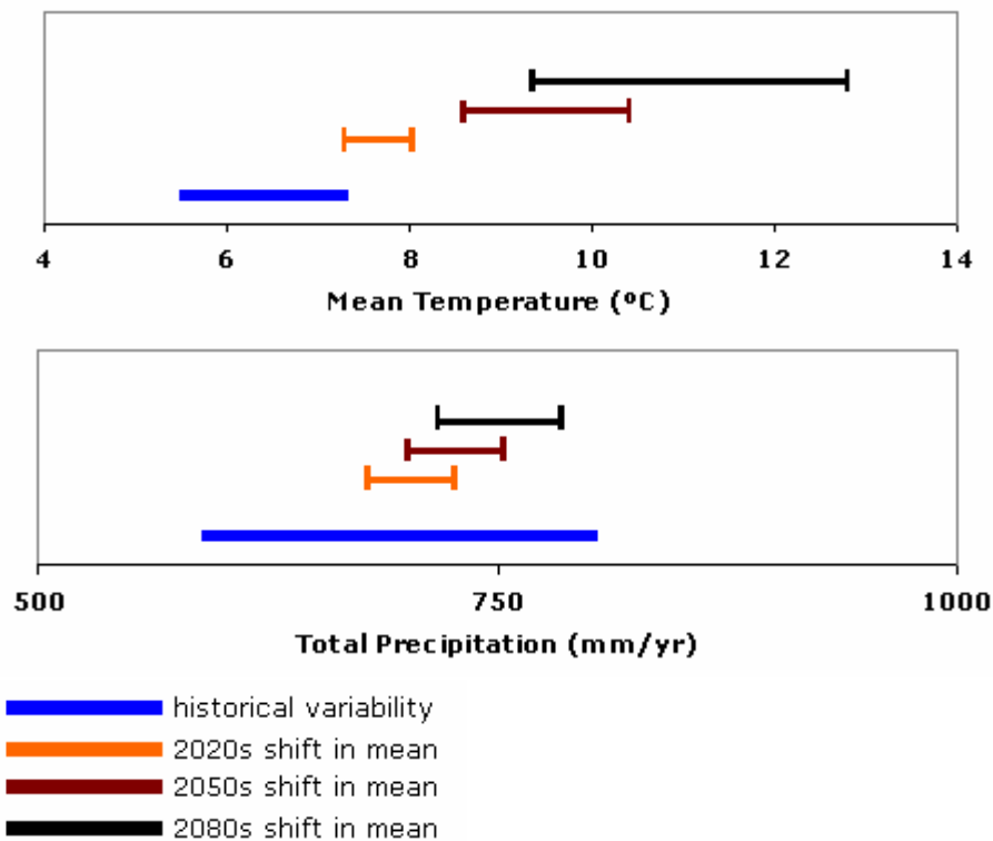
Figure 3.7: Comparison of 20th century observed variability to 21st century range of shift in mean for the Basin. Adapted from similar figure by the University of Washington, Climate Impacts Group. Blue bars for historical variability based on \pm 1 standard deviation from observed 1913-2002 record. Future shifts from 10th and 90th percentiles.
