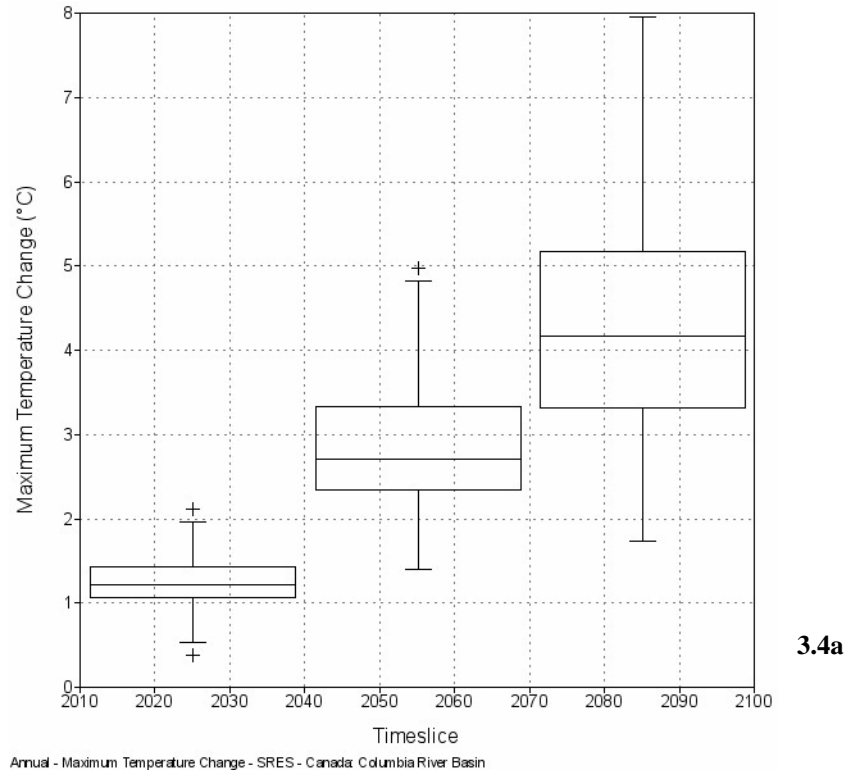
Figure 3.4: (a) Annual maximum temperature projections for the Basin 2020s, 2050s, and 2080s
