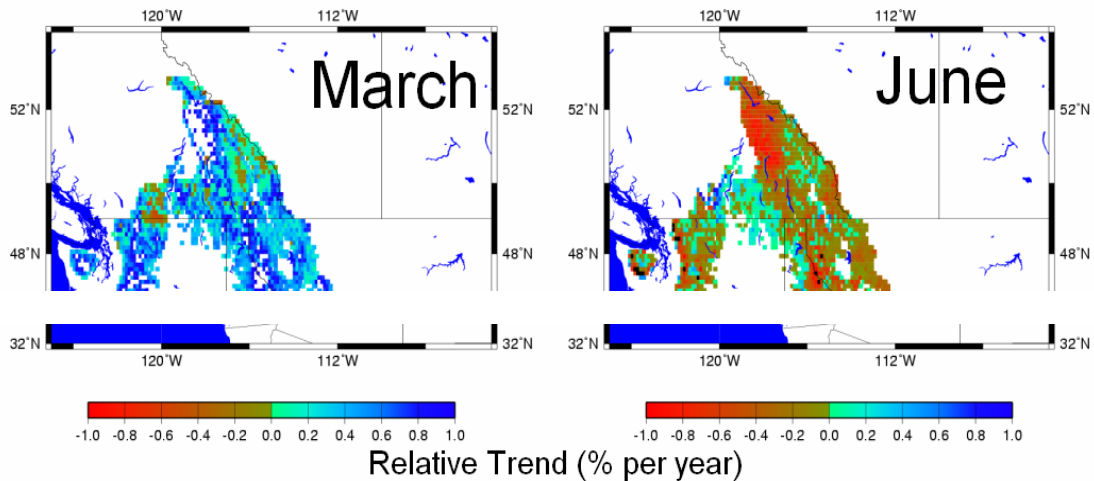
Figure 4.2: Trends in simulated proportion of annual streamflow in each month from 1974-2003 (cells > 50 mm of SWE on April 1) from VIC model. Source: Climate Impacts Group, University of Washington.
