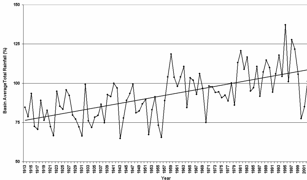
Figure 3.8: (a) Annual rainfall record and trend for the Basin 1913-2002 (b) Annual rainfall trends and confidence intervals for each station and Basin average 1913-2002
