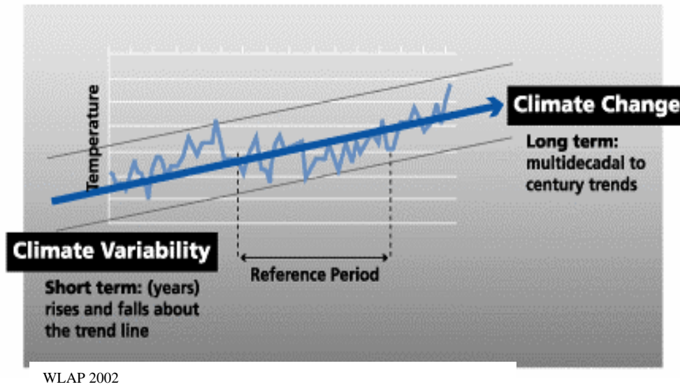
Figure 2.2: Time scales of climate variability and climate change
