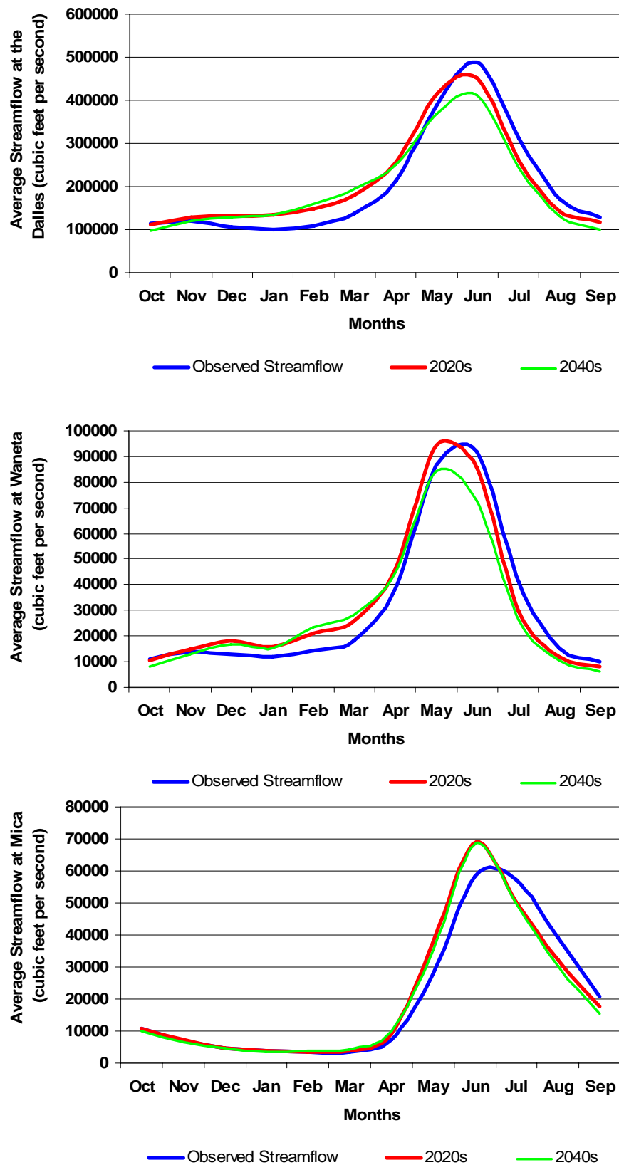
Figure 4.3: Observed and projected future streamflow for selected sites on the Columbia River. Source: Climate Impacts Group, University of Washington.
