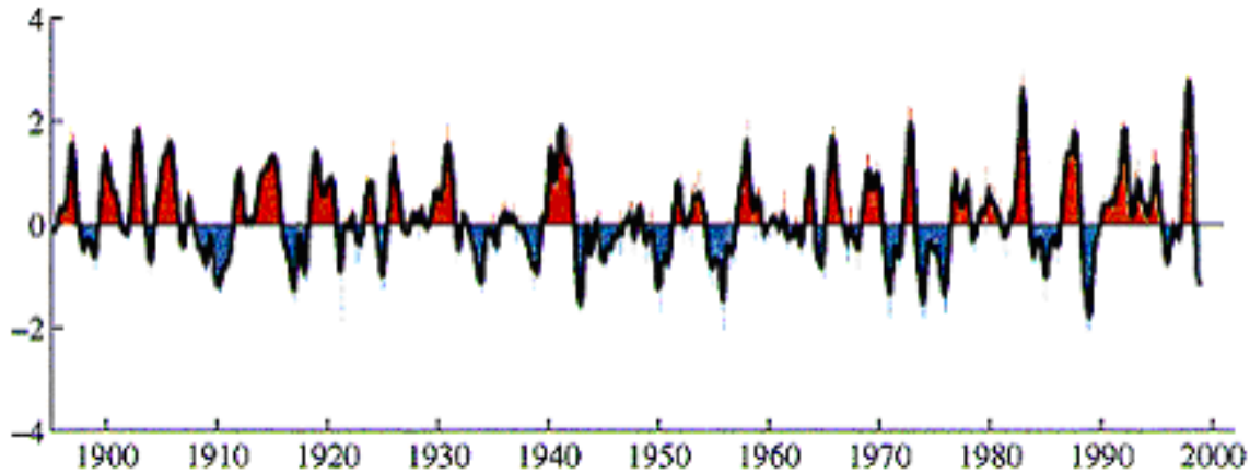
Figure 2.3: Monthly Average Values for the Niño 3.4 ENSO Index. Positive (red) index values indicate an El Niño event. Negative (blue) values indicate a La Niña event. 5
