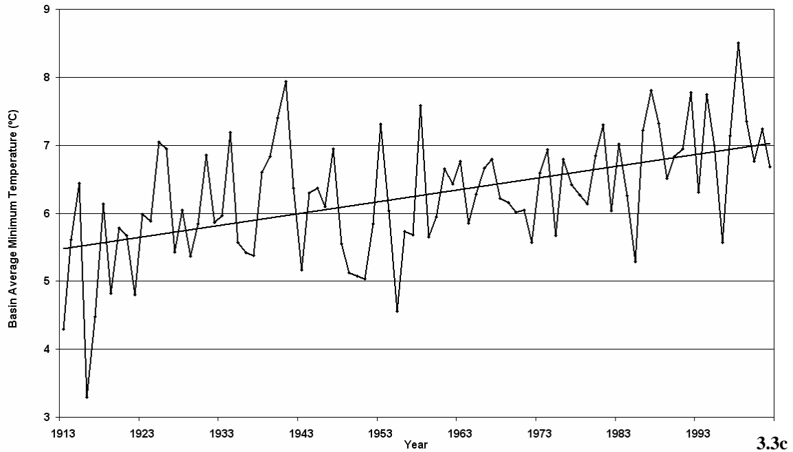
Figure 3.3: (c) Annual minimum temperature record and trend for the Basin 1913-2002 (d) Annual minimum temperature trends and confidence intervals for each station and Basin average 1913 – 2002.
