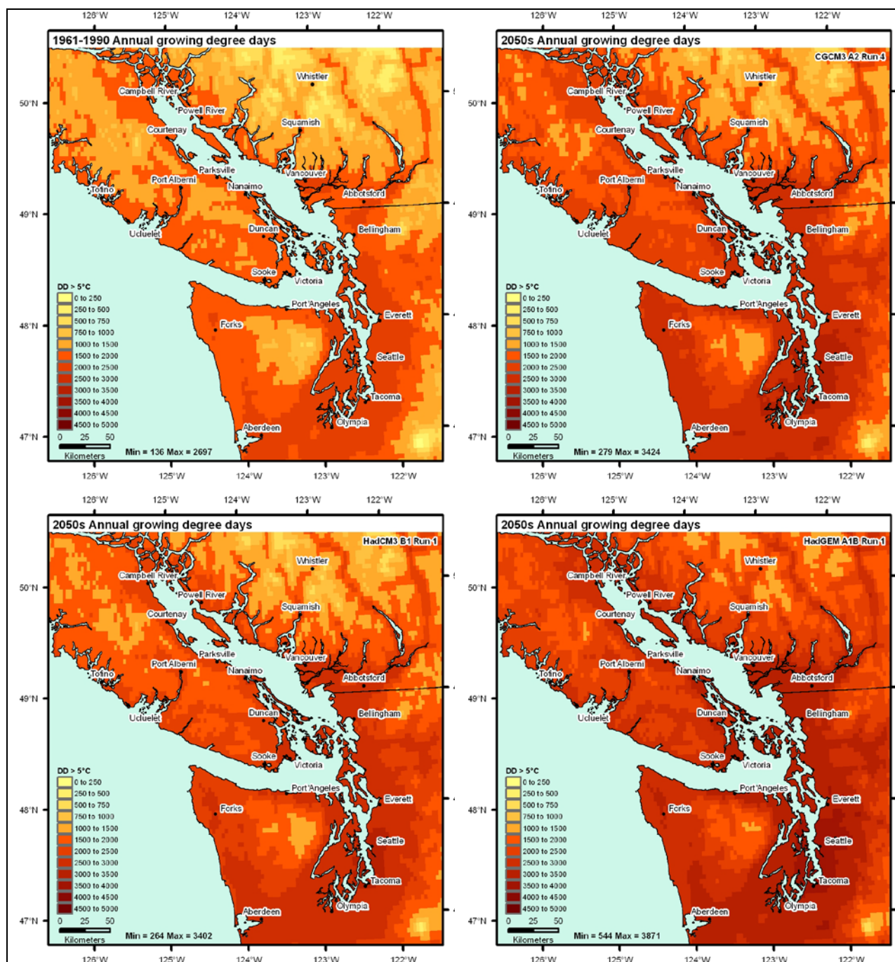
Figure 9: Annual growing degree days for 1961-1990 historical baseline (top left) and future 2050s projections according to CGCM3 A2 run 4 (top right), HadCM3 B1 run 1 (bottom left) and HadGEM A1B run 1 (bottom right).
