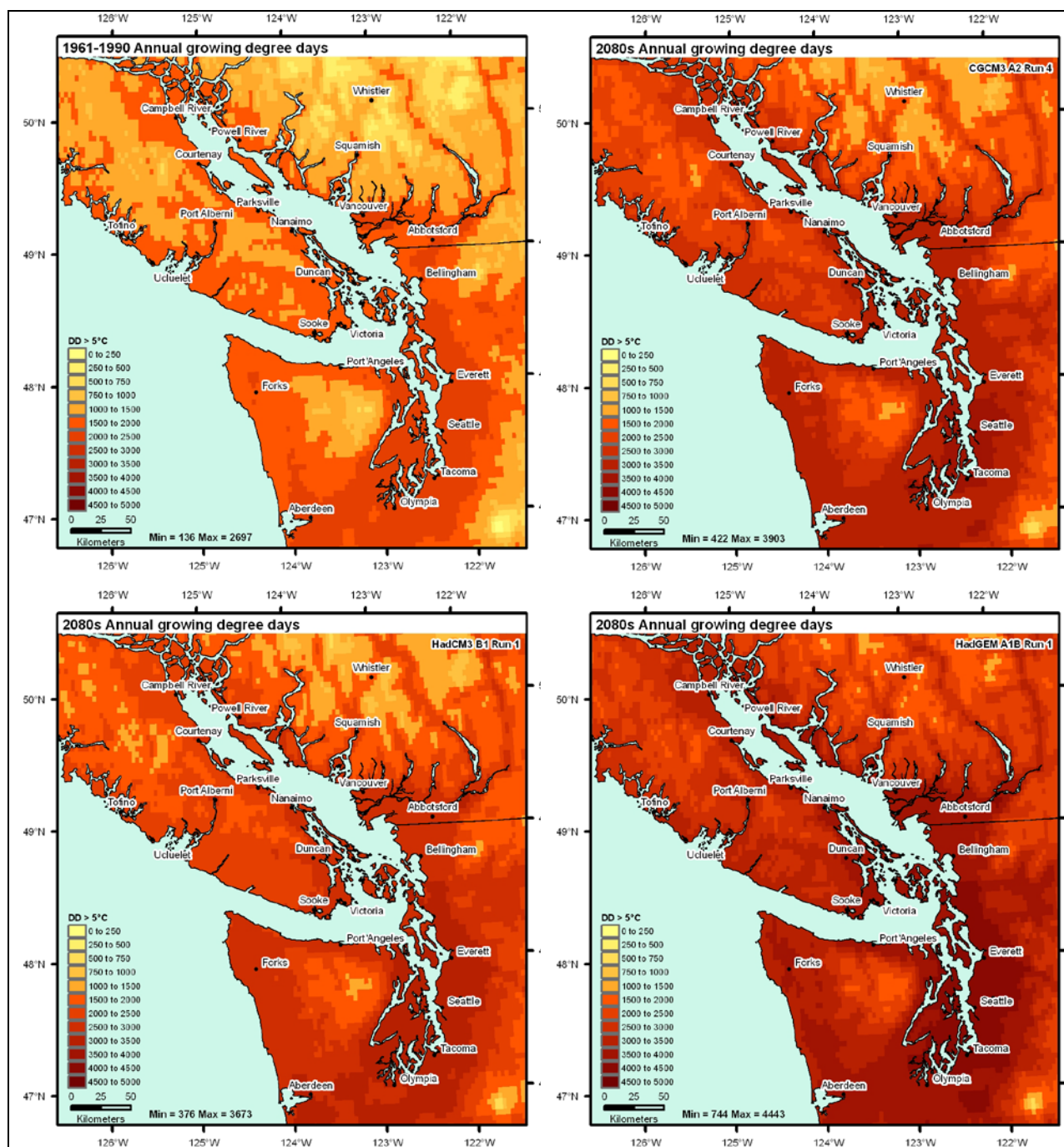
Figure 10: Annual growing degree days for 1961-1990 historical baseline (top left) and future 2080s projections according to CGCM3 A2 run 4 (top right), HadCM3 B1 run 1 (bottom left) and HadGEM A1B run 1 (bottom right).
