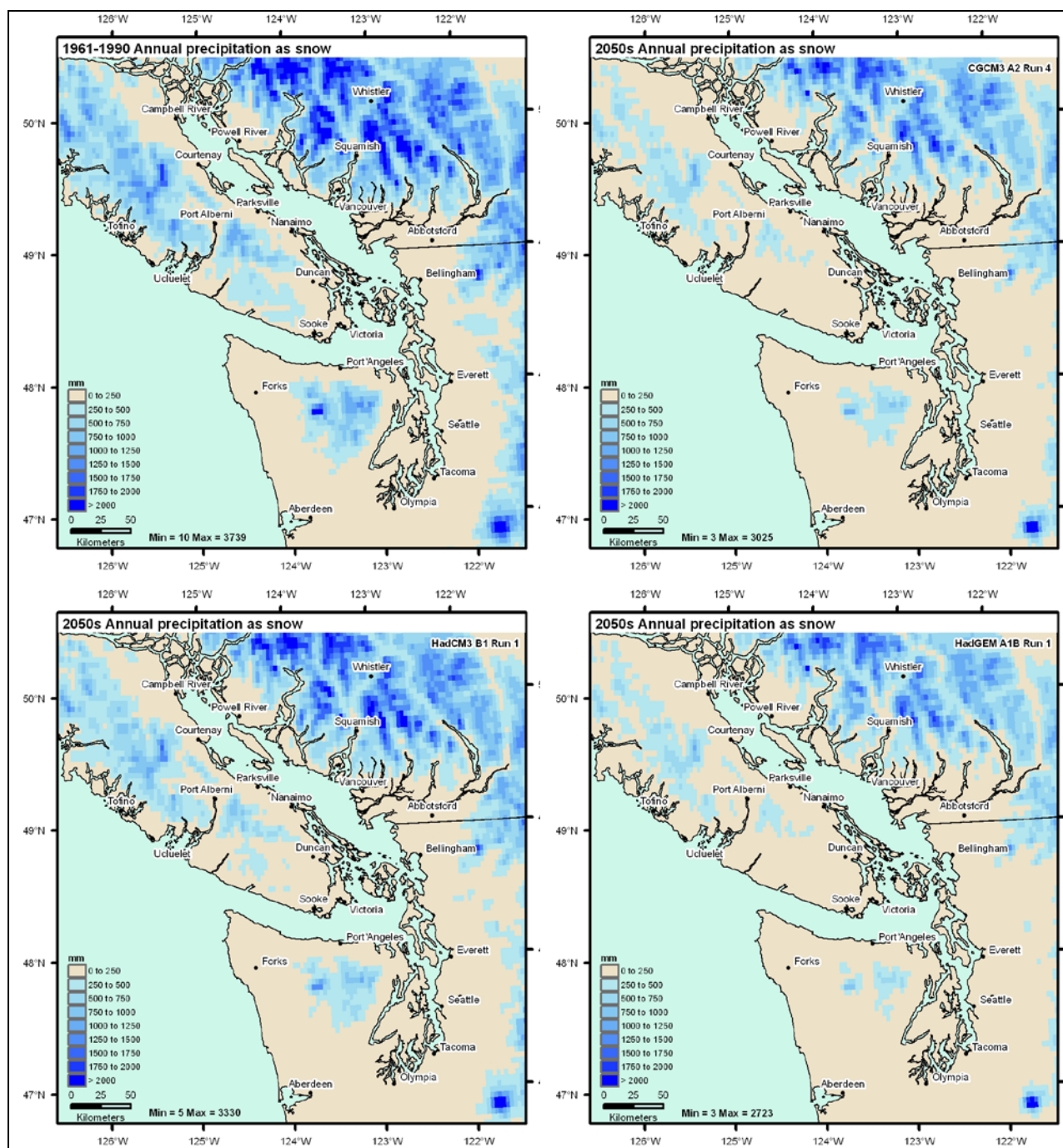
Figure 7: Annual precipitation as snow for 1961-1990 historical baseline (top left) and future 2050s projections according to CGCM3 A2 run 4 (top right), HadCM3 B1 run 1 (bottom left) and HadGEM A1B run 1 (bottom right).
