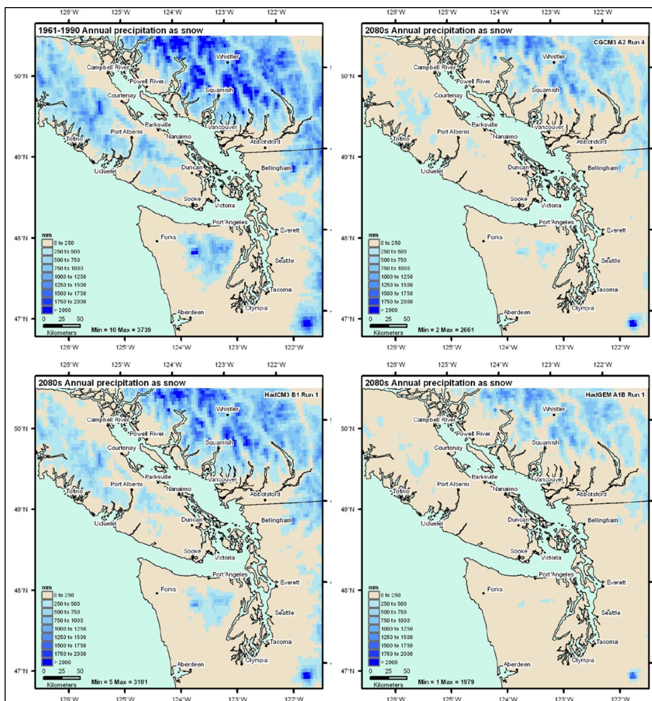
Figure 8: Annual precipitation as snow for 1961-1990 historical baseline (top left) and future 2080s projections according to CGCM3 A2 run 4 (top right), HadCM3 B1 run 1 (bottom left) and HadGEM A1B run 1 (bottom right).
